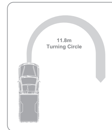
*Single Cab illustrated – load bed length is 1805mm on Club Cab
