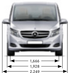
(2,057 with mirrors folded)
