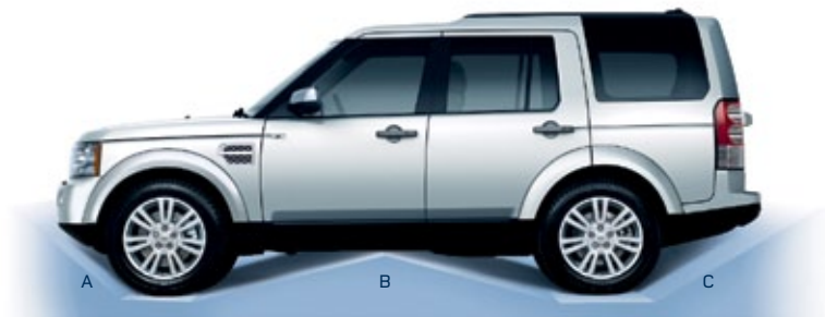
Off-road Geometry A B C Approach Angle 36.2° 27.3° 29.6° Ramp Break Over Angle Departure Angle Off-road ride height
